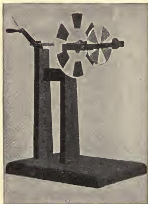
Fig. 48. Model representing the action of the semi-circular canals.
